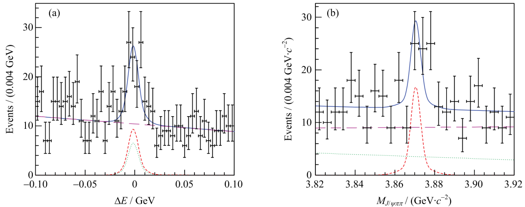
Fig. 3 Projections of the (\Delta E, M_{J/\psi\pi\pi}) fit for the B^\pm \rightarrow X(3872)K_S^0\pi^\pm decay mode
