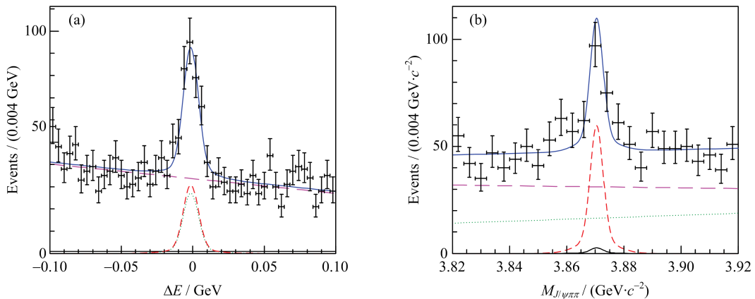
Fig. 1 Projections of the (\Delta E, M_{J/\psi\pi\pi}) fit for the B^0 \rightarrow X(3872)K^+\pi^- decay mode
