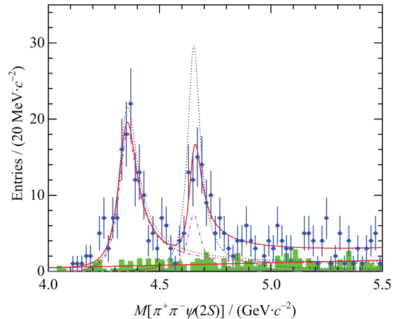
Fig. 5 The \pi^+ \pi^- \psi(2S) invariant-mass distributions and the simultaneous fit results described in the text
