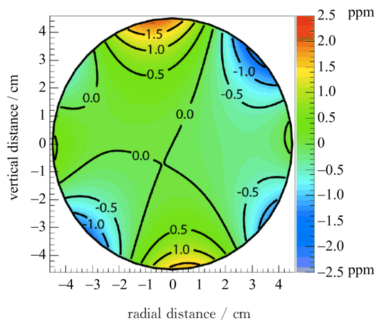
Fig. 5 A contour plot of the magnetic field averaged over azimuth of the ring at 0.5 ppm intervals
