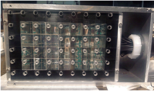
Fig. 11 PbF 2 crystal array for a beam test
