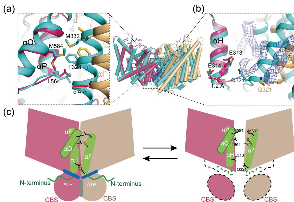
Fig. 3. Disease-related residues on the dimer interface of HsCLC-7. (a, b) Detailed interaction changes between CLC-7-flexible (purple and orange) and CLC-7-stable (cyan). Key residues are shown as sticks. Lipids in (a) are omitted for clarity. (c) Working model of HsCLC-7 regulation by the cytoplasmic domain-mediated dimer change. The left panel shows the CLC-7 state with a well-folded cytoplasmic domain consisting of CBS domains, the N-terminus, and ATP. The right panel shows the CLC-7 state with disordered N-terminus and CBS domains.
