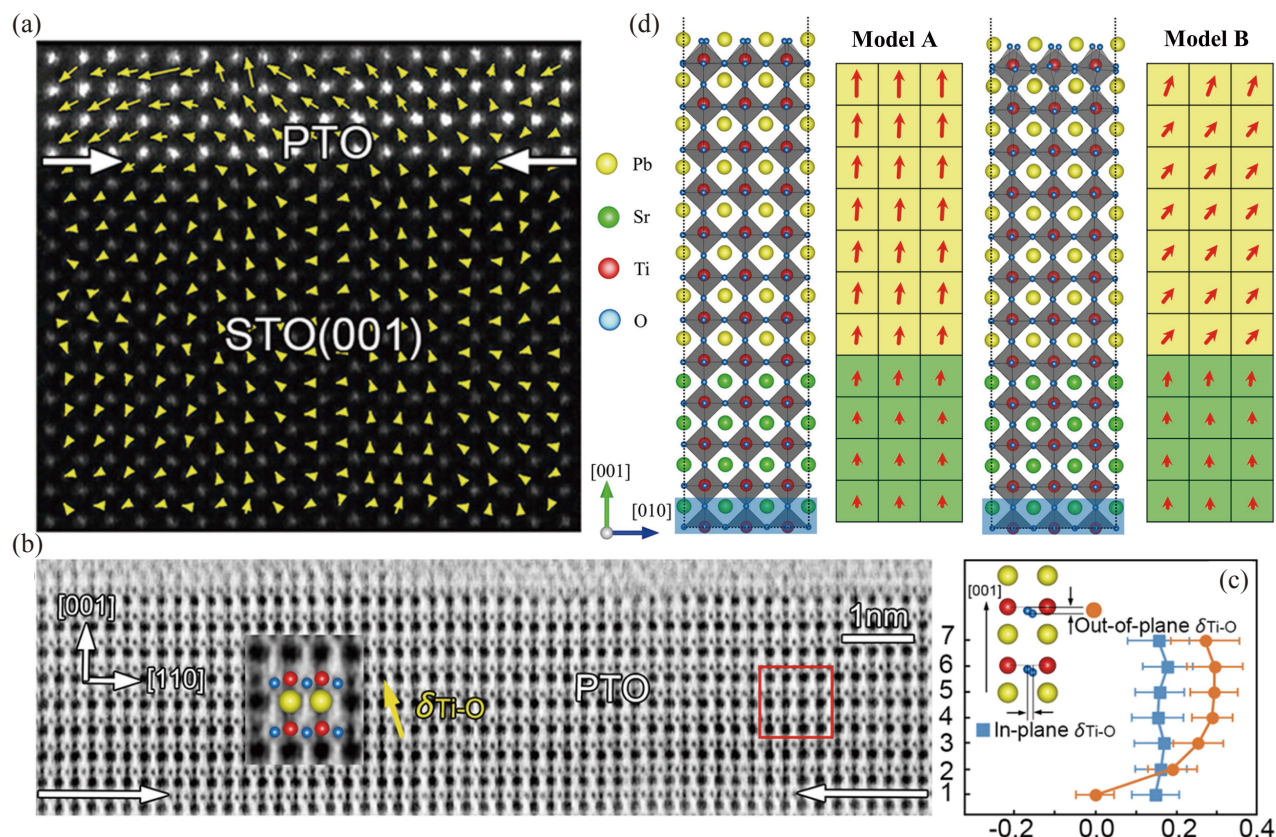
Fig. 6. Rotation of electric polarization induced by oxygen octahedral rotation. (a) HAADF-STEM image of the 1.6 nm thick PTO film and the electric polarization distribution. (b) are the ABF-STEM results. (c) Magnitude ( \delta_{\text{Ti-O}} ) of \text{Ti}^{4+} deviated from the oxygen octahedra center in- and out-of- plane of the 3.2 nm PTO film, respectively. (d) First-principles calculation results, where Model A and Model B give the relaxed atomic configuration with and without AFD, respectively. And the results of the electrical polarization simulation are shown on the right. Figure taken from Ref. [39].
