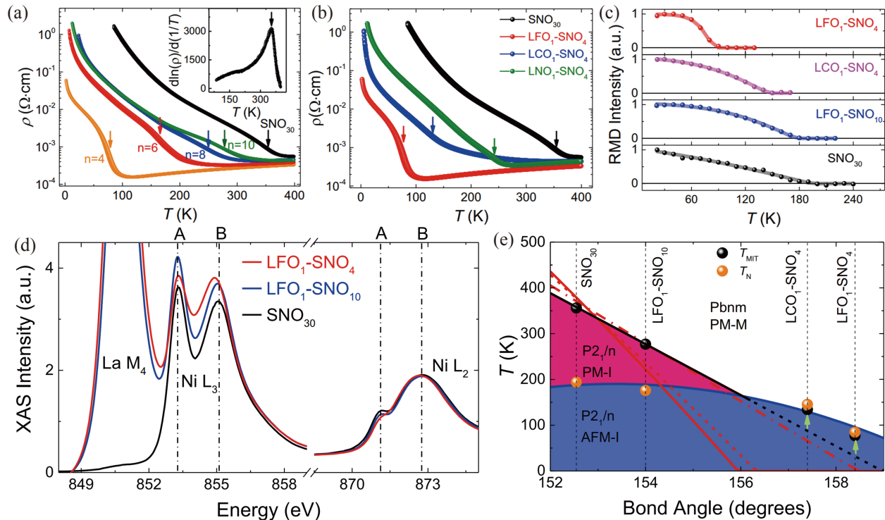
Fig. 4. MIT in nickelate superlattices triggered by oxygen octahedral coupling. (a) \rho - T curves of \text{LFO}_1\text{-SNO}_n ( n = 4\text{--}10 ) superlattices and 30 u.c. SNO film, and the inset shows the first derivative d\ln\rho/d(1/T) of the \text{SNO}_{30} film. (b) \rho - T curves of \text{SNO}_4 superlattices constructing with LFO, LCO and LNO. (c) Temperature dependent intensity of (1/4, 1/4, 1/4) magnetic Bragg reflection peak. (d) X-ray absorption spectra (XAS) of Ni L 2,3 edge of nickelate superlattices with different thicknesses at 22 K. (e) Temperature phase diagram of nickelate superlattices as a function of the mean Ni–O–Ni bond angle. Figure taken from Ref. [72].
