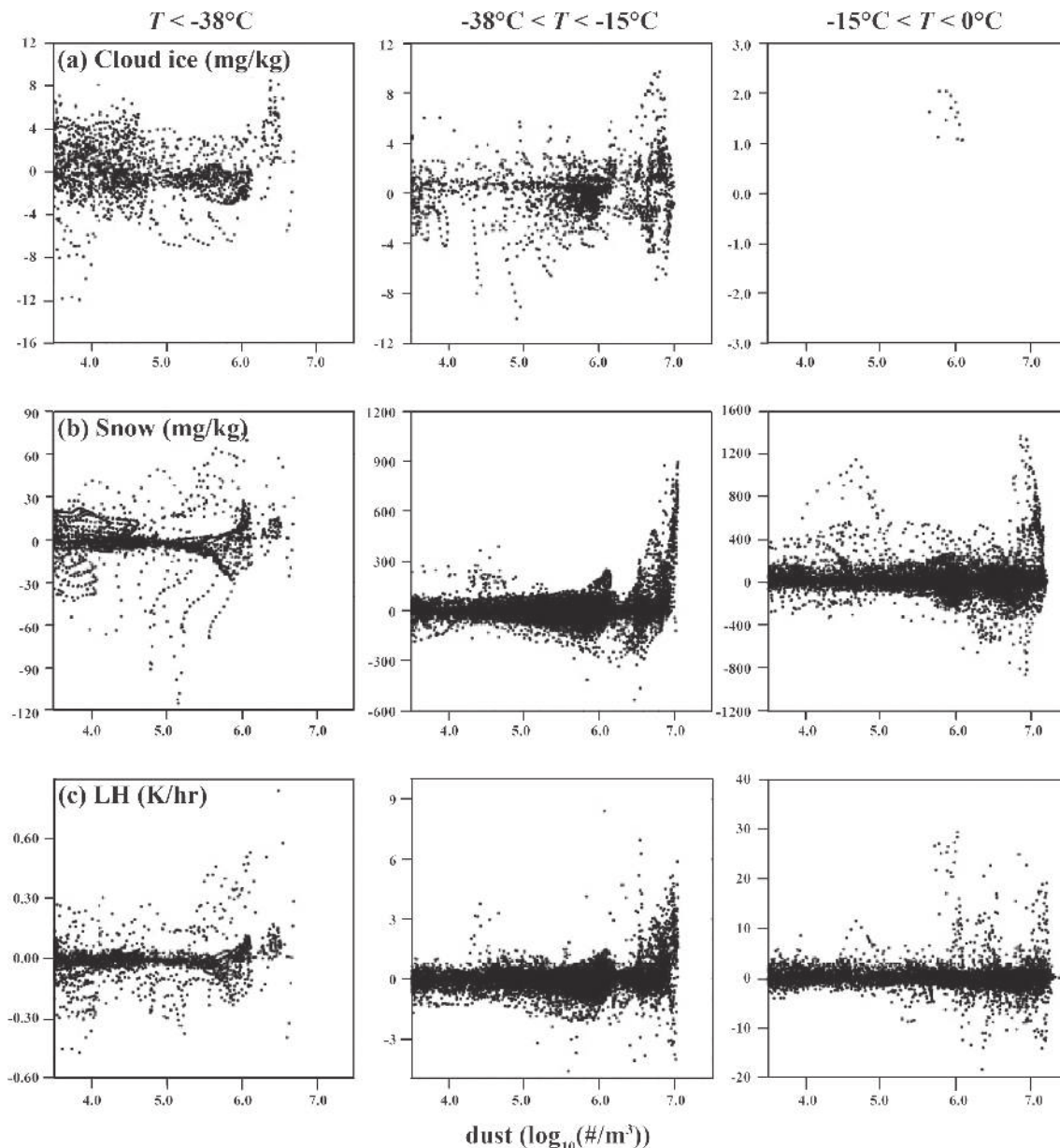
Fig. 9. The difference of cloud ice (up row), snow (mid row) and latent heating (bottom row) between WRF-DS and WRF-ND at temperature colder than -38^{\circ}\text{C} , -38^{\circ}\text{C} < T < -15^{\circ}\text{C} and warmer than -15^{\circ}\text{C} as functions of dust number concentration.
