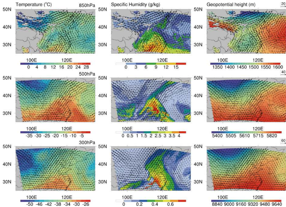
Fig. 1. The spatial pattern of air temperature (left column), specific humidity (central column) and geopotential height (right column) at 850 hPa (top row), 500 hPa (middle row) and 300 hPa (bottom row) at 8:00 UTC on 2017-05-03 derived from Climate Forecast System Reforecast product.
