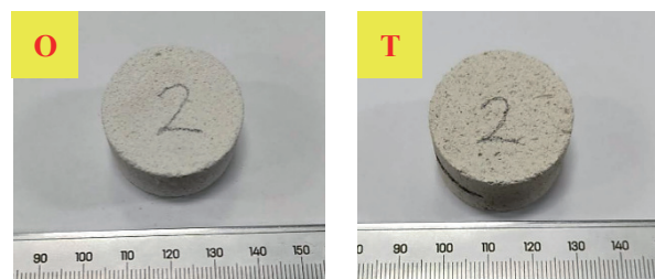
Fig. 2. Photographs of SHPB tests samples.
